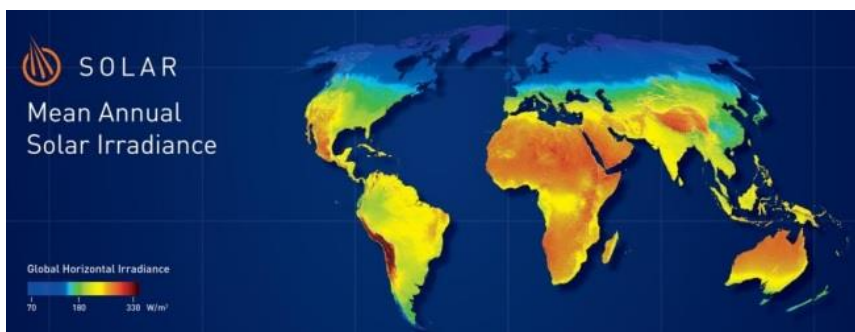
Figure 3. World solar resource map [18]
