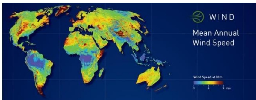
Figure 4. World wind resource map [18]
