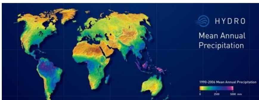
Figure 5. World hydro resource map [18]
